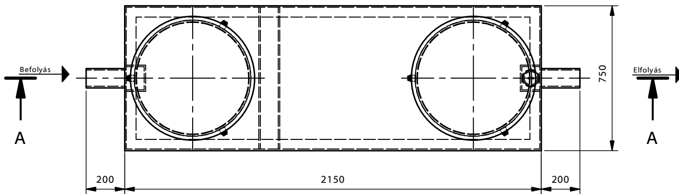
PARCO 4-P ( 1 : 50 )
